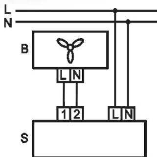
Controller wiring diagram
